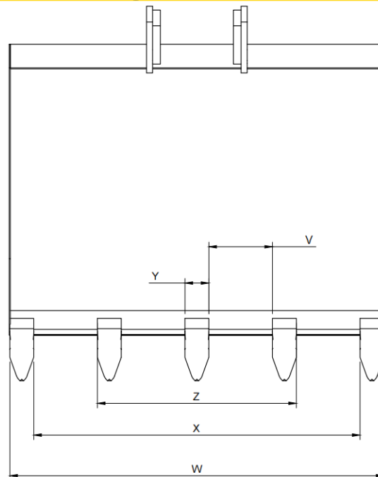
BUCKET WITH 5 TEETH
